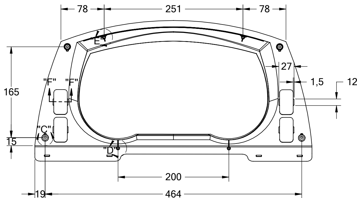
CORTE "BB" "BB" CROSS SECTION Scale 1:4
