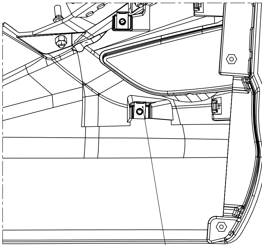
DETALHE "B" "B" DETAIL Scale 1:3
