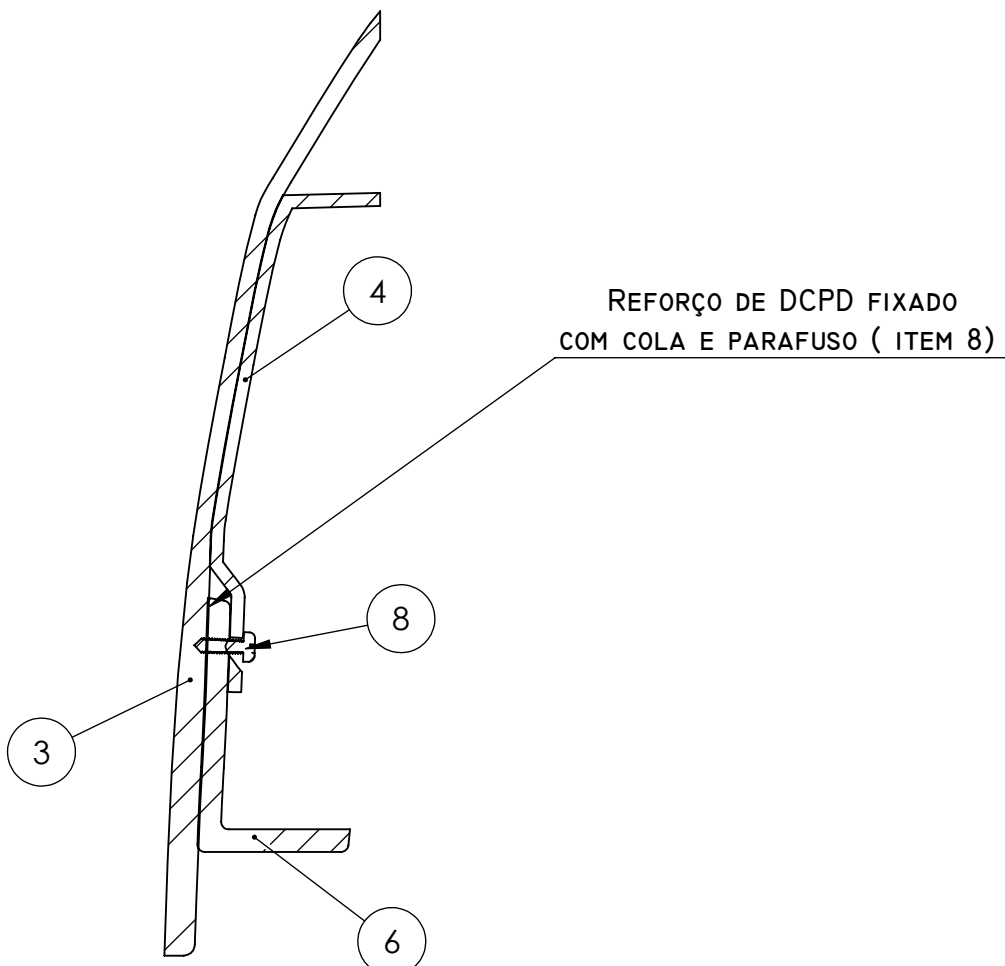
SECCAO "FF" "FF" SECTION Scale 1:2
