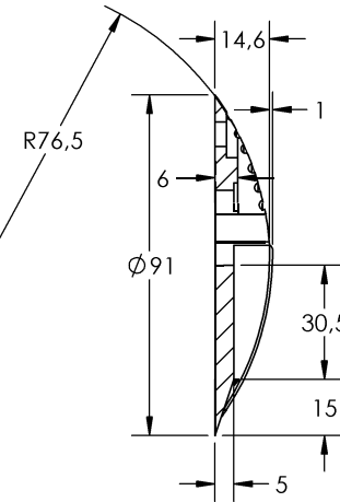
CORTE "BB" "BB" CROSS SECTION
