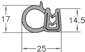
SECCAO "BB" "BB" SECTION Scale 1:1
