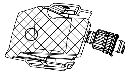
CORTE "AA" "AA" CROSS SECTION Scale 1:3
