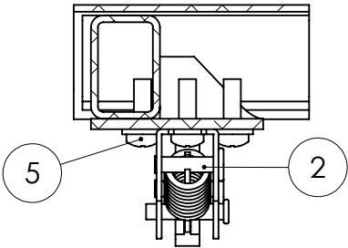
SECCAO "CC" "CC" SECTION Scale 1:2
