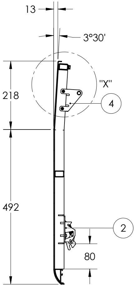
SECCAO "AA" "AA" SECTION
