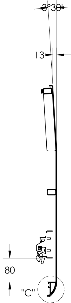
SECCAO "BB" "BB" SECTION
