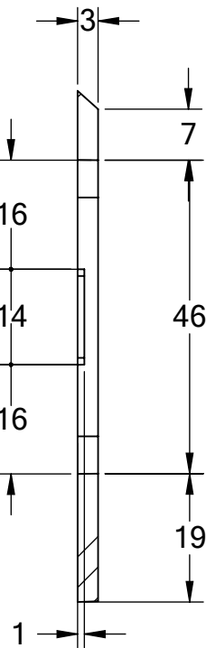
SECCAO "BB" "BB" SECTION Scale 1:1
