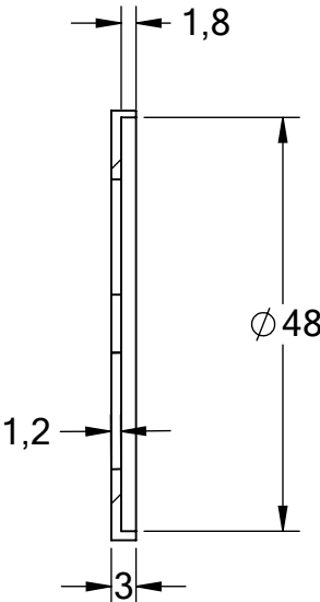
SECCAO "DD" "BB" SECTION Scale 1:1
