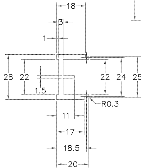
SECCAO "DD" "DD" SECTION Scale 1:1
