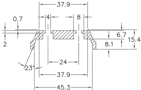
SECCAO "CC" "CC" SECTION Scale 1:1
