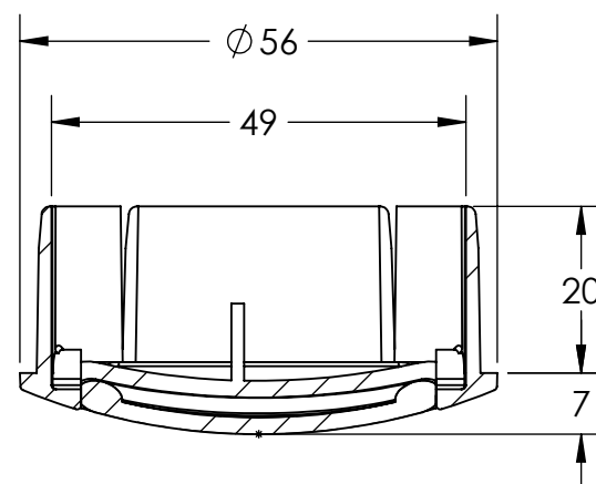
CORTE "BB" "BB" CROSS SECTION Scale 1:1
