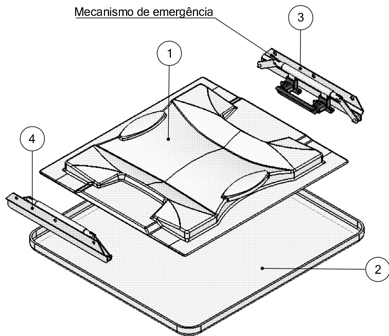
VISTA ISOMÉTRICA EXPLODIDA EXPLODED ISOMETRIC VIEW
