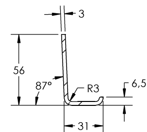
SECCAO "BB" "BB" SECTION Scale 1:2
