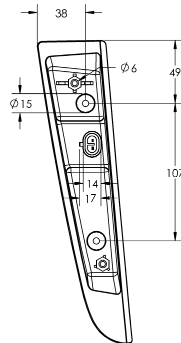
VISTA "A" "A" VIEW Scale 1:2
