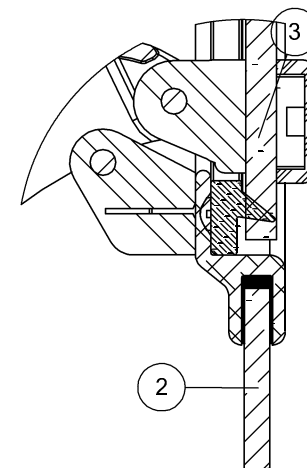
DETALHE "C" "C" DETAIL Scale 1:1
