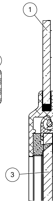
DETALHE "B" "B" DETAIL Scale 1:1
