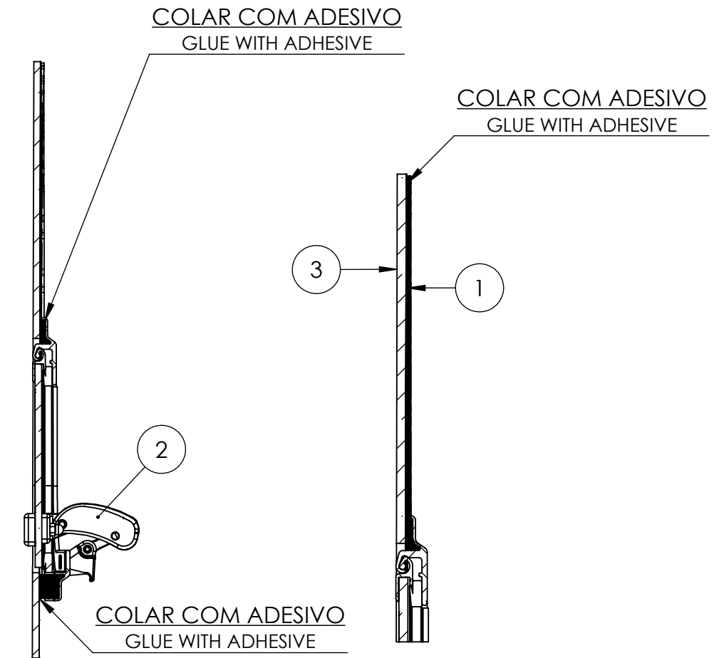
CORTE "BB" "BB" CROSS SECTION Scale 1:3
