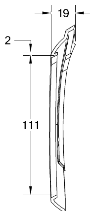
SECCAO "AA" "AA" SECTION Scale 1:1
