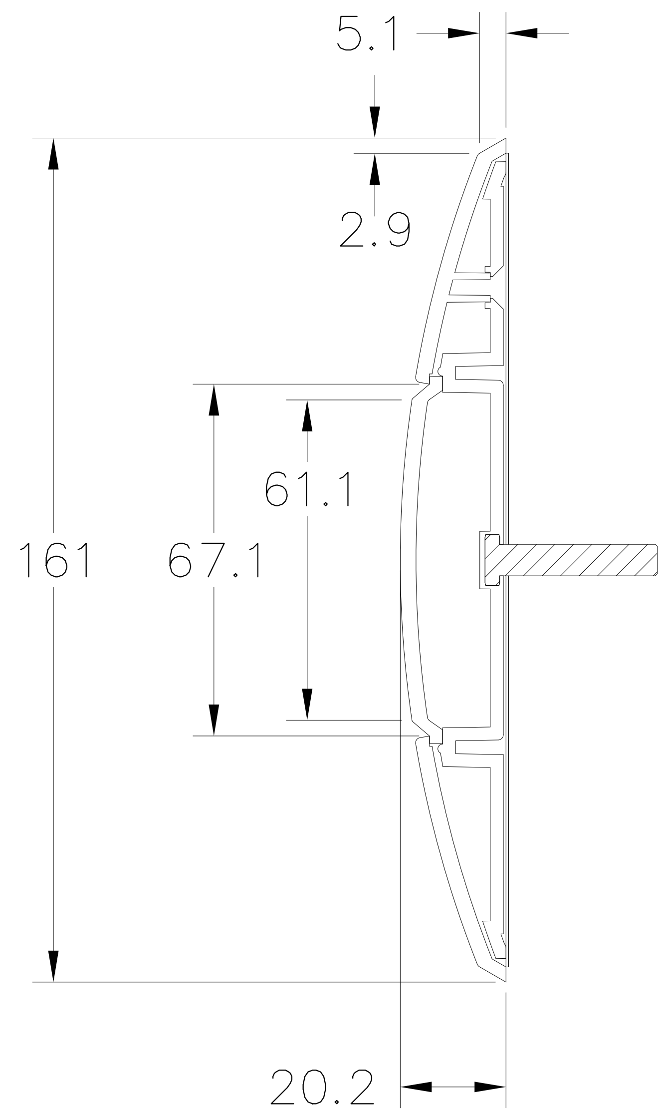
SECCAO "AA" "AA" SECTION Scale 1:1
