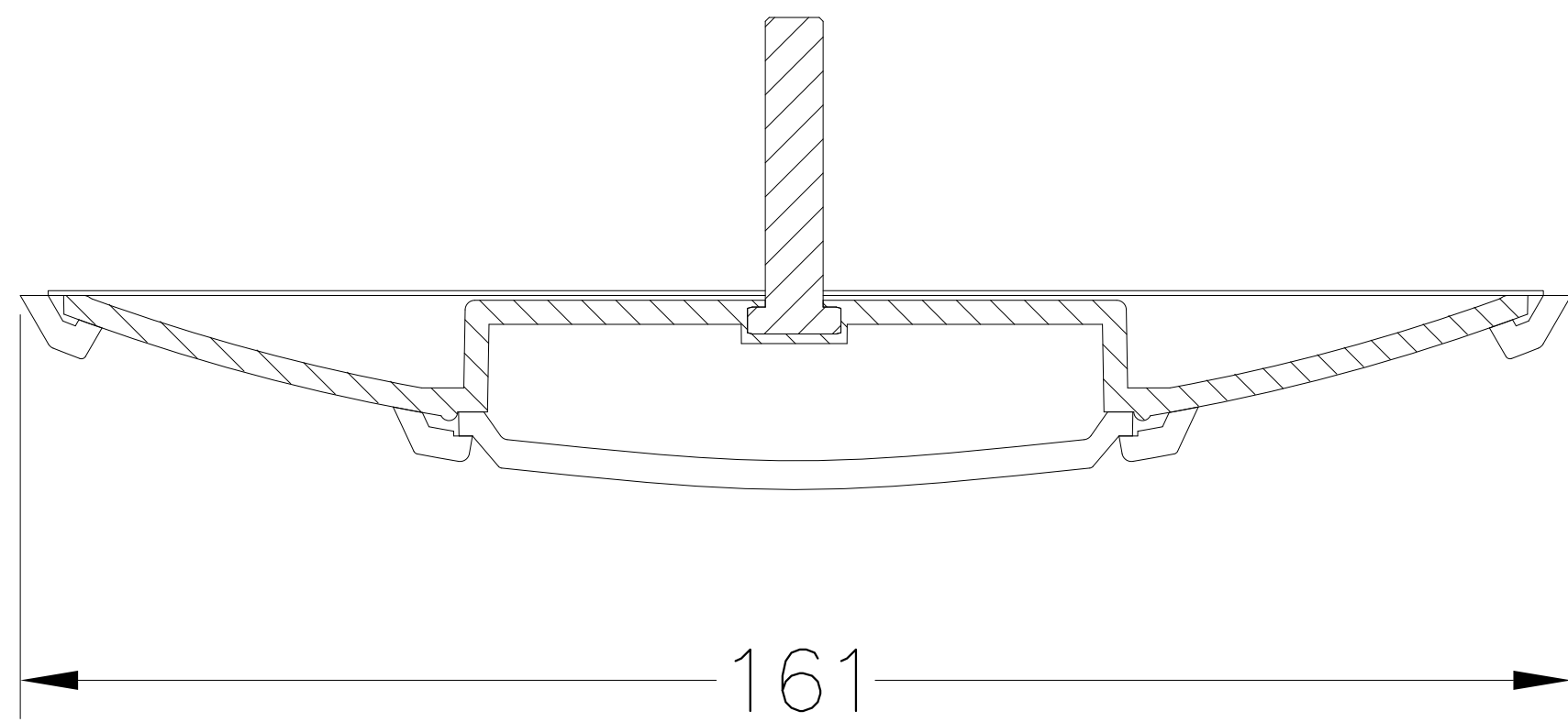
SECCAO "BB" "BB" SECTION Scale 1:1
