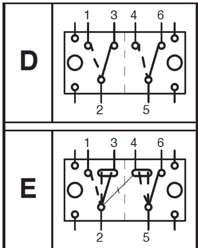
Circuit Diagram
