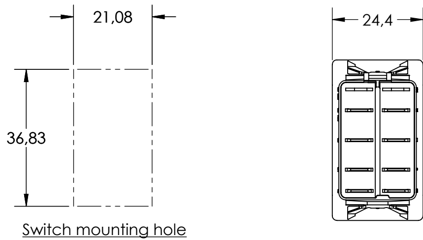
Switch mounting hole
