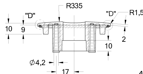
CORTE "BB" "BB" CROSS SECTION Scale 1:1
