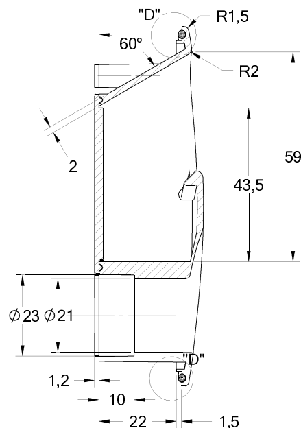
CORTE "AA" "AA" CROSS SECTION Scale 1:1
