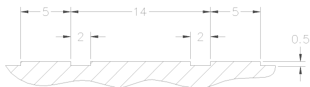
SECCAO "AA" "AA" SECTION Scale 4:1
