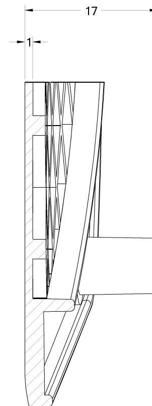
SECCAO "BB" "BB" SECTION Scale 3:1
