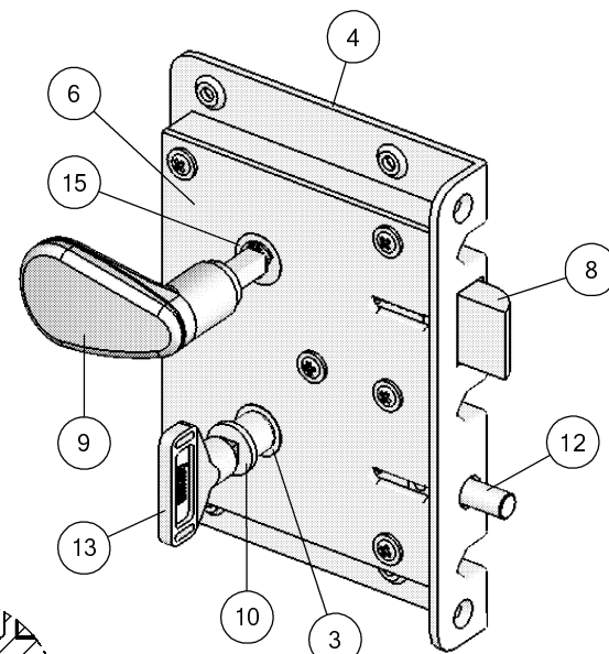
VISTA ISOMETRICA ISOMETRIC VIEW
