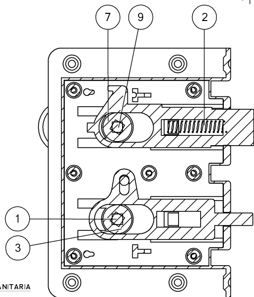
CORTE "AA" "AA" CROSS SECTION Scale 1:2
