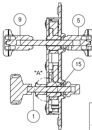
CORTE "BB" "BB" CROSS SECTION Scale 1:2
