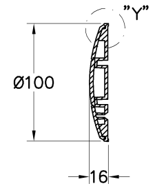
SECCAO "AA" "AA" SECTION Scale 1:3
