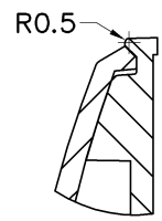
DETALHE "Y" "Y" DETAIL Scale 1:5:1
