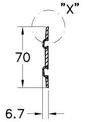
SECCAO "BB" "BB" SECTION Scale 1:3
