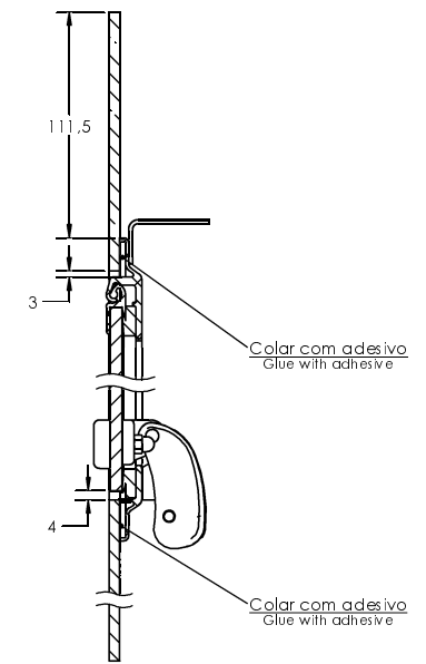
CORTE "BB" "BB" CROSS SECTION Scale 1:2
