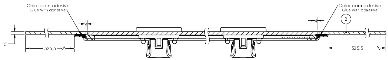
CORTE "AA" "AA" CROSS SECTION Scale 1:2
