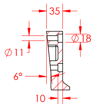
SECCAO "JJ" "JJ" SECTION Scale 1:4
