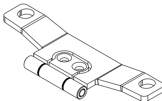
VISTA ISOMÉTRICA ISOMETRIC VIEW
